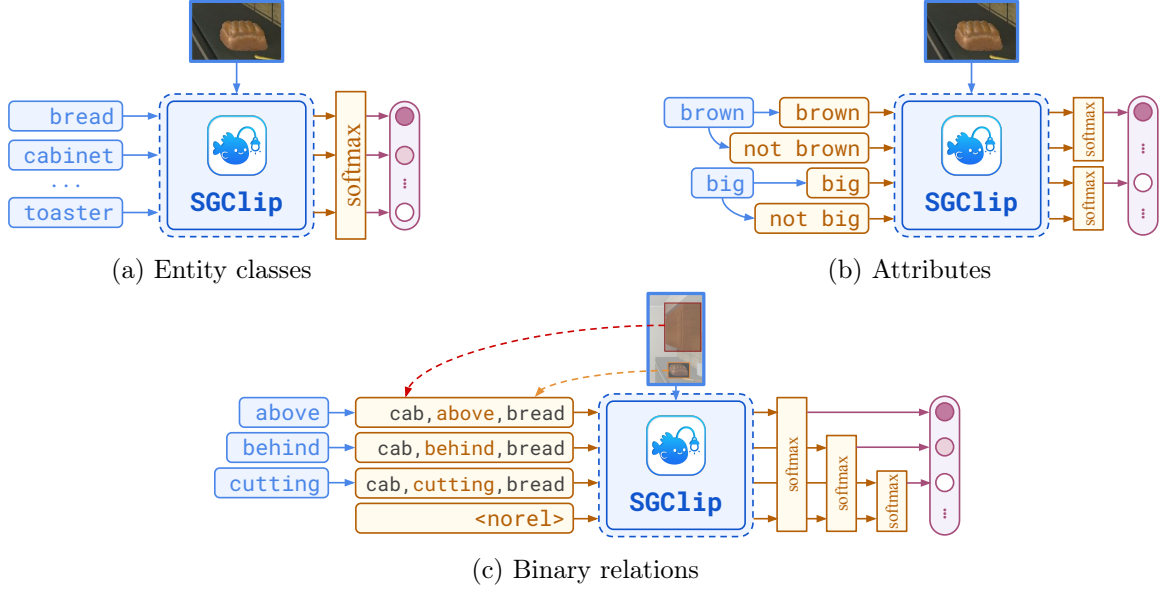
Figure 6.8: Illustration of the inference modes of SGClip for three types of concepts: entity classes, attributes, and binary relations. While the model stays the same, the three inference modes perform different pre- and post-processing for a more accurate semantic estimation of probabilities.
