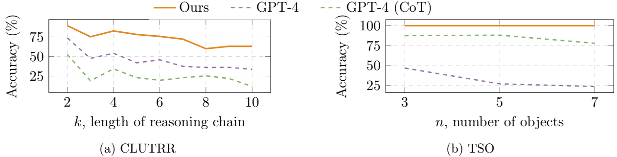
Figure 5.10: Systematic generalizability comparisons on the CLUTRR and TSO datasets.
