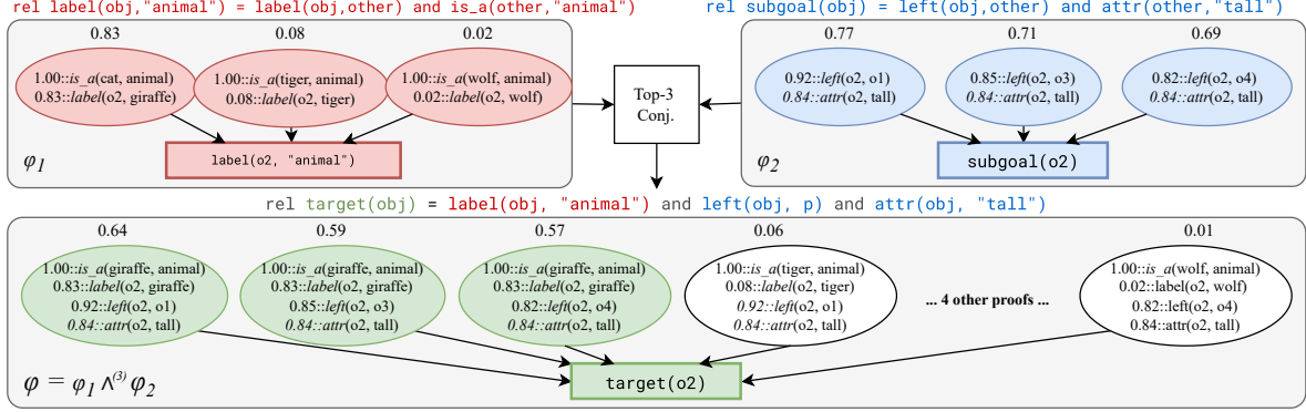
Figure 3.13: Illustration of top- k conjunction using k = 3 . Each ellipse represents a proof of the fact shown in the box. Given the top 3 proofs for each of “ \text{label}(o_2, \text{"animal"}) ” and “ \text{subgoal}(o_2) ”, we wish to derive the top 3 proofs for their conjunction, “ \text{target}(o_2) ”. The join yields 9 possible proofs. After computing the likelihood for each of the 9 proofs, we keep the top 3 most likely ones (green ellipses) and discard the rest (white ellipses).
